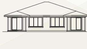
REAR ELEVATION
