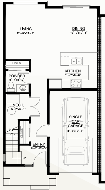
MAIN FLOOR PLAN
